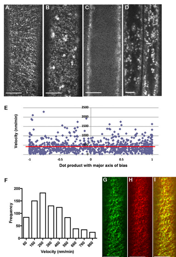
Fig. 3. CSI1 is localized to CESA-like particles in dark-grown hypocotyls cells. (A–D) Optical sections of epidermal cells in 3-d-old dark-grown hypocotyls expressing RFP-CSI1 (A and C) and YFP-CESA6 (B and D). Focal planes of the plasma membrane (A and B) and lower cortex (C and D) are shown. (Scale bar: 5 μm.) (E) Plot of RFP-CSI1 particle velocity vs. its dot product (i.e., scalar product; see Methods) with the direction of bias. Red line indicates the linear regression of the plot. A slope of 0 indicates no bias in direction. (F) Histogram of measured RFP-CSI1 particle velocities. The mean is 416 nm/min ( n = 917 ). (G–I) Localization of GFP-CESA3 (G), RFP-CSI1 (H), and merge (I). (Scale bar: 5 μm.)
