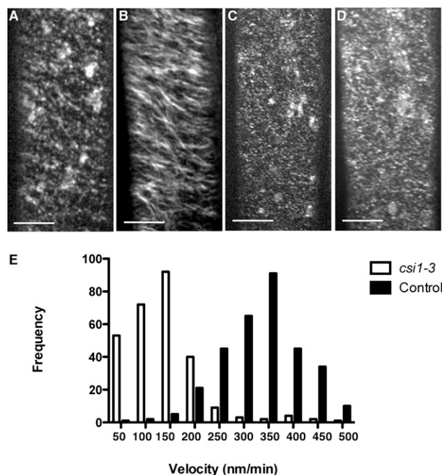
Fig. 4. YFP-CESA6 dynamics are altered in csil-3 mutants. YFP-CESA6 localization in dark-grown hypocotyls cells is shown in wild-type plants (A and B) and csil-3 mutants (C and D). (A) A single optical section acquired at the plane of plasma membrane in wild-type plants. (B) Average of 61 frames (duration: 2 min; 2-s interval) showing movement of labeled particles along linear trajectories. (C) Single optical section of YFP-CESA6 in csil-3 mutant. (D) Average of 61 frames (duration: 2 min; 2-s interval) in csil-3 mutant. (Scale bars: 5 \mu m.) (E) Histogram of measured particle velocities. The mean velocity is 365 nm/min in control plants ( n = 318 ) and 132 nm/min in csil-3 mutants ( n = 225 ).
