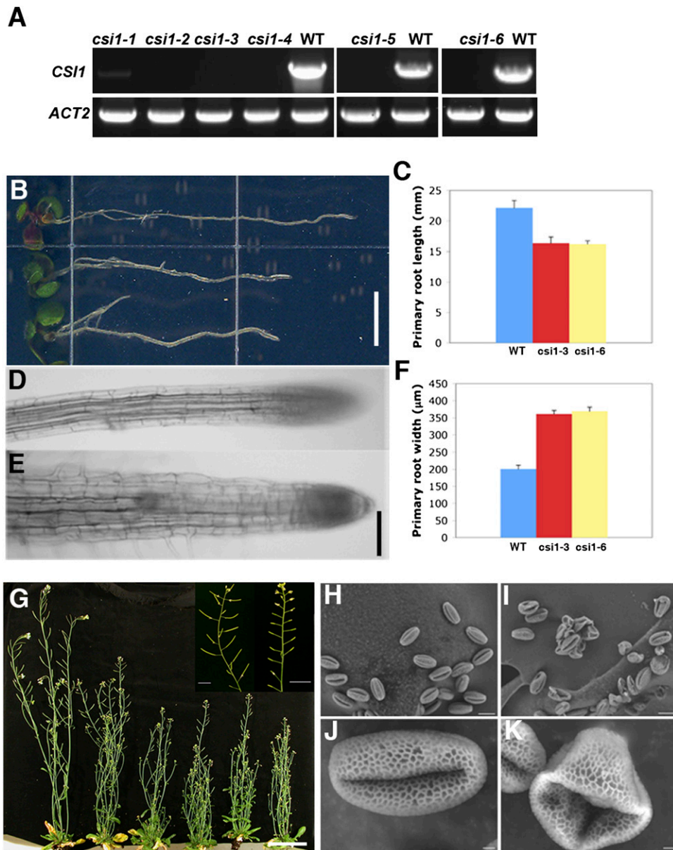
Fig. S3. Morphology of csi1 mutants. (A) RT-PCR analysis of CSI1 mRNA expression in various transfer DNA (T-DNA) insertion lines in 1-wk-old seedlings. ACTIN2 was used as control. WT, Columbia-0. (B) Eight-day-old Col-0 (Top), csi1-3 -mutant (Middle), and csi1-6 -mutant (Bottom) seedlings were grown on 1/2 MS supplemented with 1% sucrose. (Scale bar: 5 mm.) (C) Quantification of primary root length in Col-0, csi1-3 -mutant, and csi1-6 -mutant seedlings. Measurement data were collected from about 50 seedlings in each genotype. (D and E) High magnification of primary root morphology in Col-0 (D) and csi1-3 -mutant plants (E). (Scale bar: 200 μm.) (F) Quantification of primary root width in Col-0, csi1-3 -mutant, and csi1-6 -mutant seedlings. Measurement data were collected from about 50 seedlings in each genotype. (G) Adult plant morphology in csi1 mutants: (Left to Right) Col-0 (wild-type) and csi1-1 , csi1-2 , csi1-3 , csi1-4 , and csi1-6 mutants. (Scale bar: 5 cm.) Insets show enlarged image of siliques from wild-type (Col-0) and csi1-3 -mutant plants. (Scale bar: 1 cm.) (H–K) Morphology of mature pollen grains in wild-type (H) and csi1-3 -mutant (I) plants examined by SEM. (Scale bar: 200 μm.) Magnified SEM images of single pollen grains from wild-type (J) and csi1-3 -mutant (K) plants. (Scale bar: 2 μm.)
