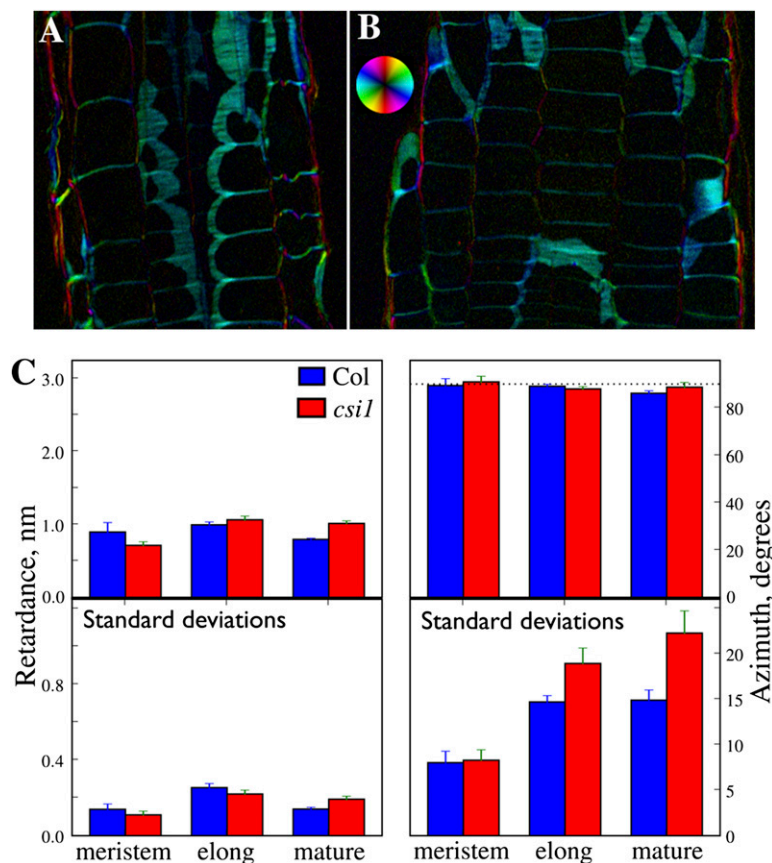
Fig. 5. Polarized light analysis of csi1 mutants. (A and B) Polarized-light micrographs of (A) wild-type and (B) csi1-1 -mutant roots. Images are of longitudinal-tangential sections through cortex and epidermis. Intensity is proportional to retardance, and color represents optical axis (azimuth) of the crystalline elements, as shown by the color wheel. Note the similar intensity and color for the two genotypes. (C) Quantification of retardance and azimuth ( 90^\circ is transverse to the root's long axis). Top panels show means \pm SEM ( n = 3 roots); bottom panels show the average SD ( n \sim 200 measurements) \pm SEM for each of the roots. Note the larger SDs for csi1-1 mutants in the elongation and mature zones.
