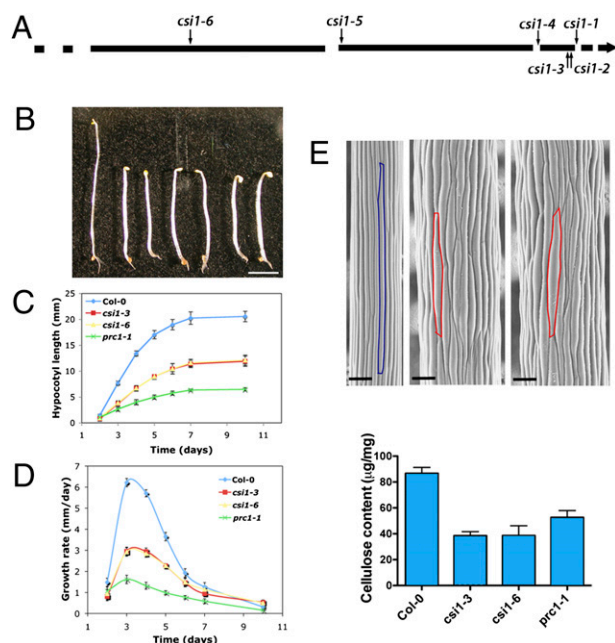
Fig. 2. CSI1 is required for normal cell expansion. (A) Schematic representation of six T-DNA insertion sites in csi1 . Exons are represented by black lines, and introns are shown by breaks. (B) Morphology of 4-d-old dark-grown seedlings: (Left to Right) Col-0 (wild-type) and csi1-1 , csi1-2 , csi1-3 , csi1-4 , csi1-5 , and csi1-6 mutants. (Scale bar: 2 mm.) (C and D) Hypocotyl length (C) and growth rate (D) of dark-grown wild-type (Col-0) plants and csi1-3 , csi1-6 , and prc1-1 mutants. Data were collected from the measurement of ~50 seedlings for each genotype. Error bars represent SE (absent error bars were obscured by symbols). (E) SEM of dark-grown hypocotyls in wild-type plants and csi1 mutants: (Left to Right) Arabidopsis thaliana Columbia (Col-0), csi1-3 , and csi1-6 mutants. Colors outline one epidermal cell. (Scale bar: 100 μm.) (F) Cellulose content was reduced in csi1 mutants. n = 5 . Error bars represent SE.
