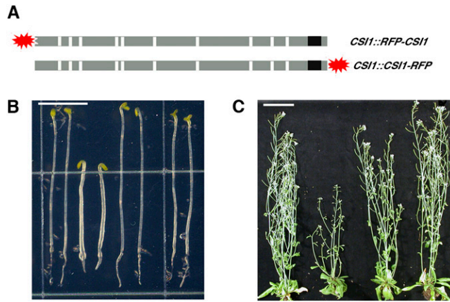
Fig. S4. Both N- and C-terminal fusion constructs complement csi1 -mutant phenotypes. (A) Schematic representation of N- and C-terminal fusion constructs. (B) Red fluorescent protein (RFP)-fusion constructs complemented csi1 -mutant phenotype in dark-grown hypocotyls. (Scale bar: 5 mm.) (C) RFP-fusion constructs complemented csi1 -mutant phenotype in adult plants: (Left to Right in B and C) wild-type (Col-0), csi1-6 mutant, CSI1::CSI1-RFP in csi1-6 mutant, and CSI1::RFP-CSI1 in csi1-6 mutant. (Scale bar: 5 cm.)
